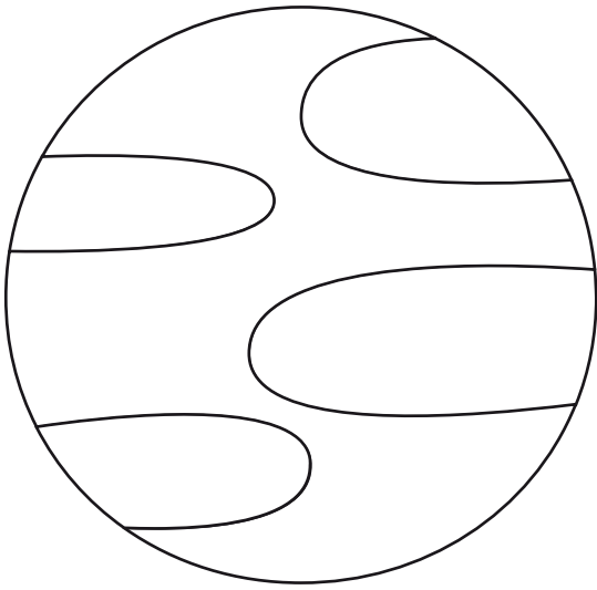
ARTIZARRA
