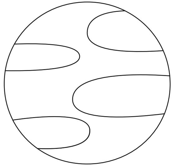
ARTIZARRA
